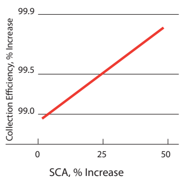
Particulate Collection Efficiency as Function of SCA
