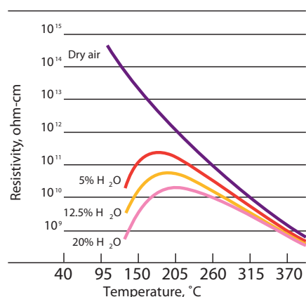
Dust Resistivity Characteristics
